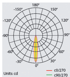
BAIKAL LU PRO-S 800W 60x60°
