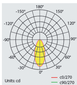
BAIKAL LU PRO-S 200W 85x135°
