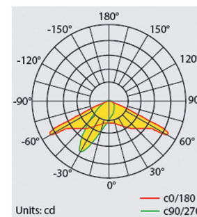
BAIKAL LU PRO-S 1000W 85x135°
