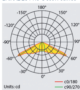
BAIKAL LU PRO-S 800W 85x45°
