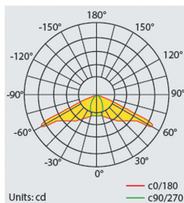
BAIKAL LU PRO-S 300W 85x45°
