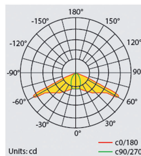
BAIKAL LU PRO-S 1000W 85x45°
