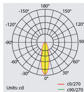
BAIKAL LU PRO-S 1000W 60x135°
