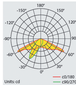
BAIKAL LU PRO-S 400W 85x135°
