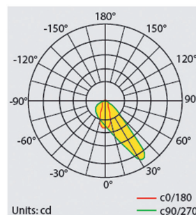
BAIKAL LU PRO-S 1000W 85x45°
