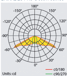
BAIKAL LU PRO-S 600W 85x45°
