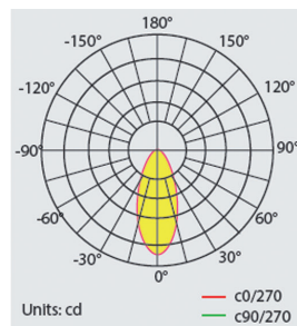
BAIKAL LU PRO-S 300W 85x135°
