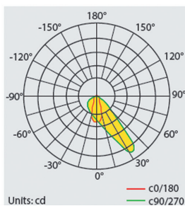
BAIKAL LU PRO-S 400W 85x45°
