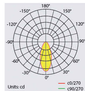
BAIKAL LU PRO-S 600W 85x135°
