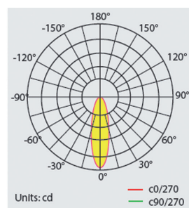
BAIKAL LU PRO-S 200W 60x135°
