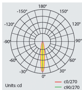
BAIKAL LU PRO-S 300W 60x60°
