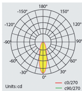
BAIKAL LU PRO-S 300W 60x135°
