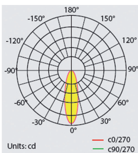
BAIKAL LU PRO-S 600W 60x135°
