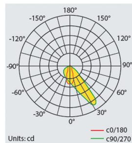
BAIKAL LU PRO-S 200W 85x45°
