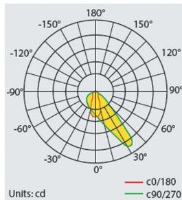
BAIKAL LU PRO-S 300W 85x45°
