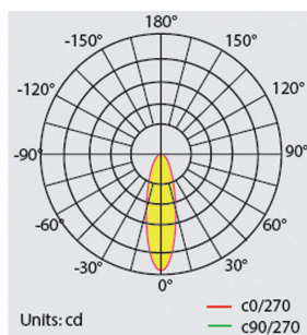
BAIKAL LU PRO-S 800W 60x135°
