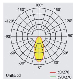
BAIKAL LU PRO-S 800W 85x135°
