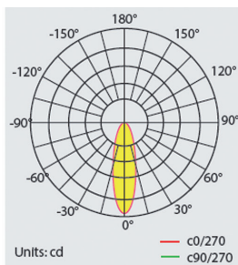
BAIKAL LU PRO-S 500W 60x135°
