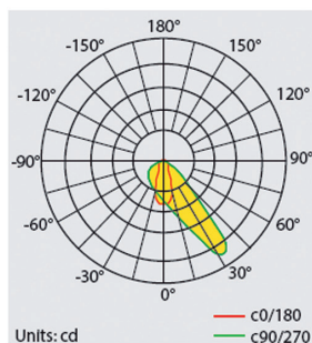
BAIKAL LU PRO-S 800W 85x45°
